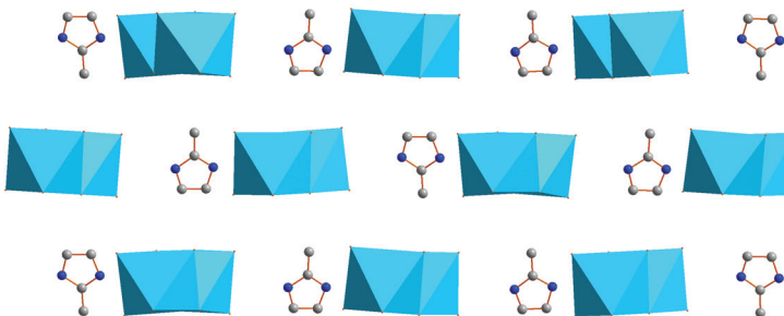
Fig. 6 Disorder of 2-MIm + in the modulated phase. (a) Down to 200 K the occupancy of two positions (which were populated with equal probability in the high-temperature phase I) may be described with harmonics which results in various occupancy of each orientation, marked here by color differentiation (a) below 200 K the switching between the positions is blocked and occupancy is better reproduced by the crenel function which defines zero or fully occupied sites.
