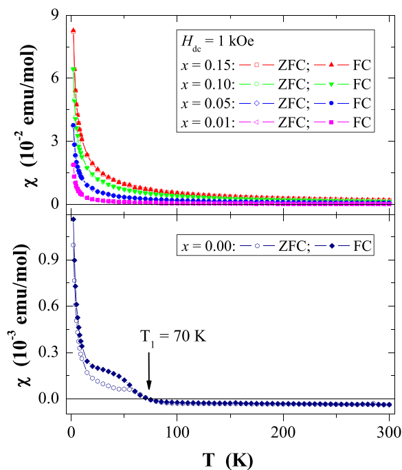
Fig. 13 ZFC and FC magnetic susceptibility ( \chi ) vs. temperature ( T ) for \text{Ca}_{1-x}\text{Mn}_x\text{MoO}_4 ( x=0.0, 0.01, 0.05, 0.10 and 0.15 ) recorded at H_{dc}=1 kOe. T_1 is the paramagnetic-diamagnetic transition for \text{CaMoO}_4
