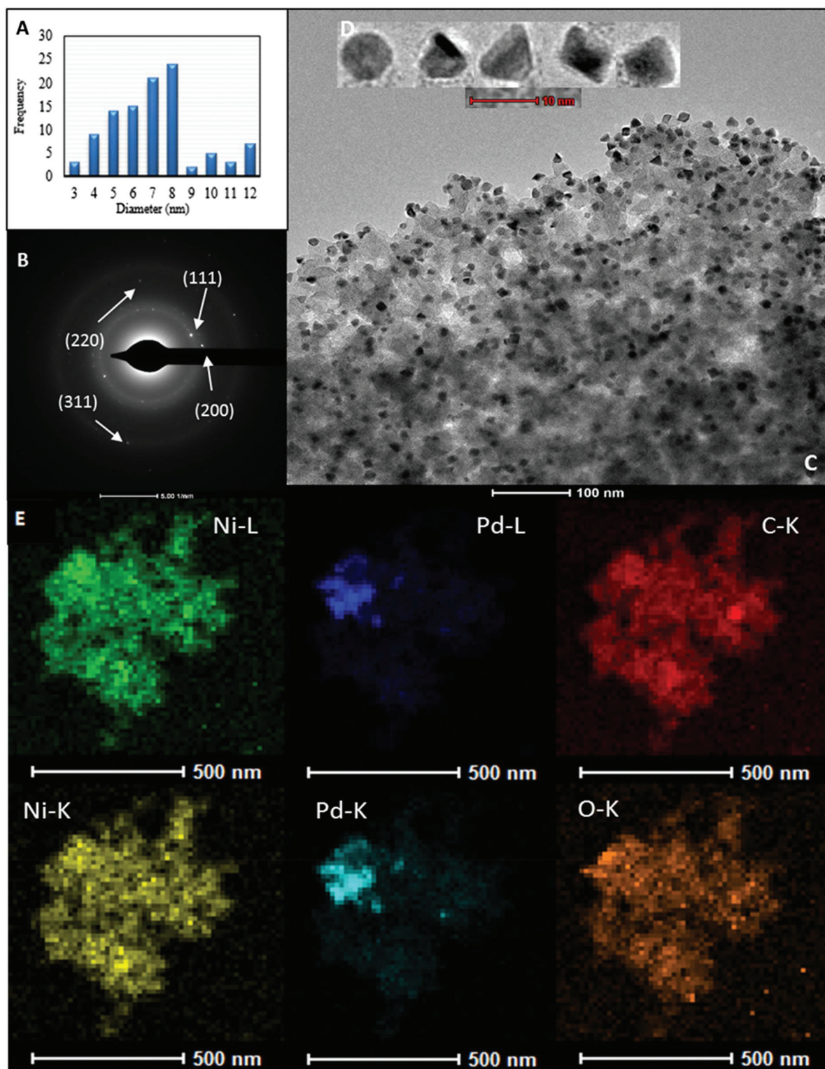
Fig. 1 (A) Histogram of Pd particle size, (B) SAED pattern of Pd nanocrystals, (C, D) TEM images of Pd NPs with different shapes found in \text{Pd}@\text{[Ni(H}_2\text{BDP-SO}_3)_2\text{]} nanocrystals, (E) EDX elemental mappings of \text{Pd}@\text{[Ni(H}_2\text{BDP-SO}_3)_2\text{]} .
